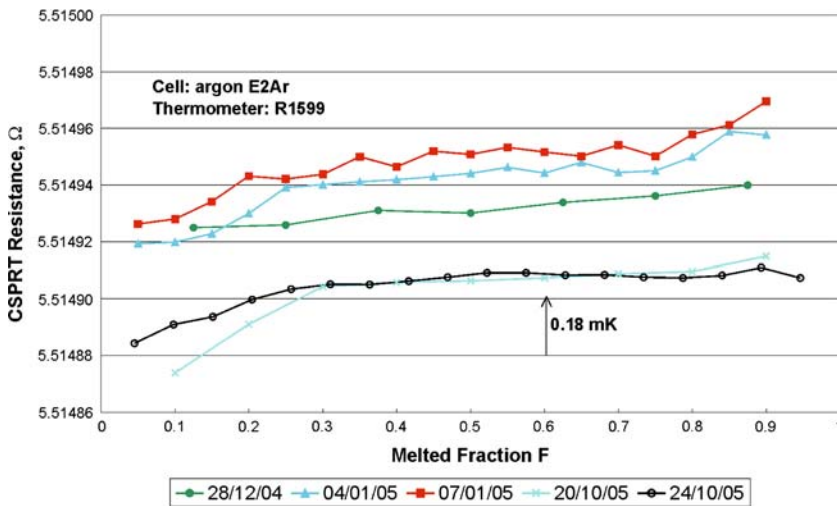
Fig. 7 Argon plateaux measured with thermometer Rosemount 1599
